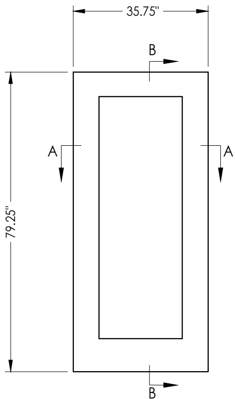
FIBERGLASS DOOR PANEL Plastpro 6' 8" Opaque/Glazed
